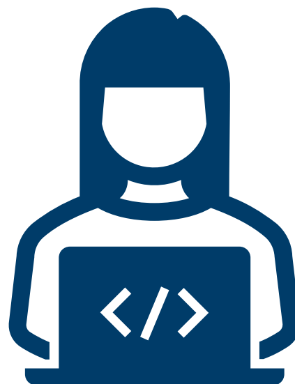
Low-Code
